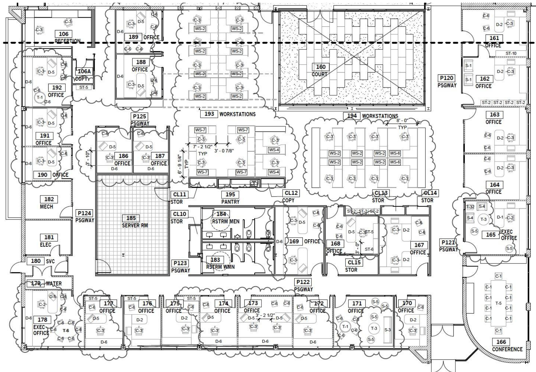
1st Floor, South
