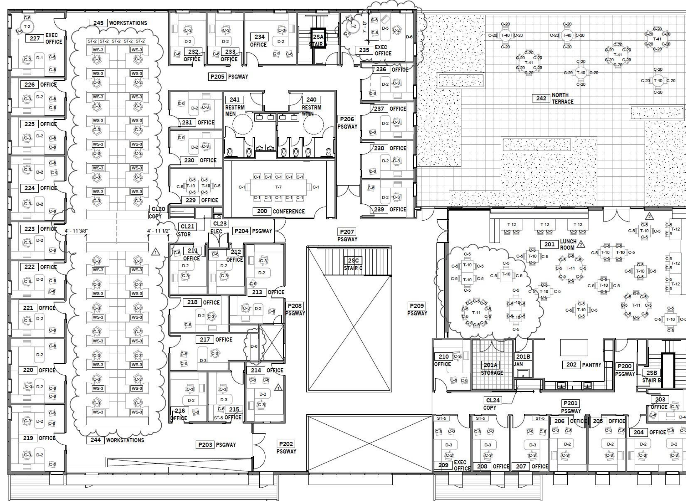
2nd Floor
